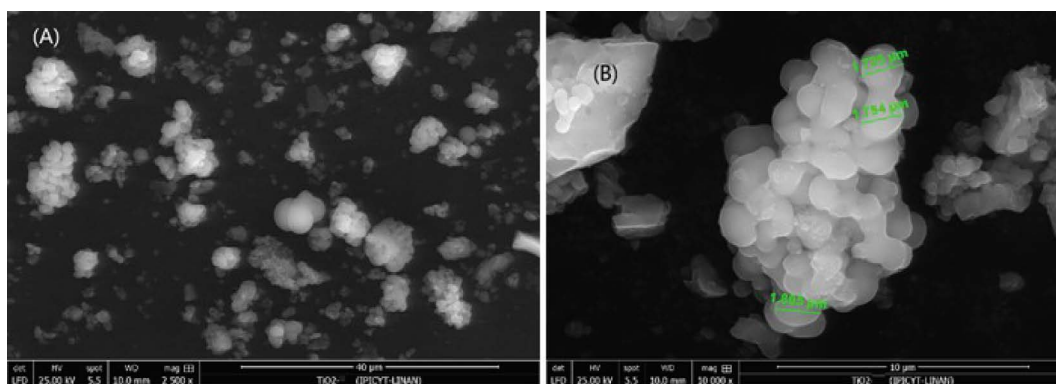
Figure 4. SEM micrographs of TiO 2 at 2500X magnification in A and 20 000X in B.
